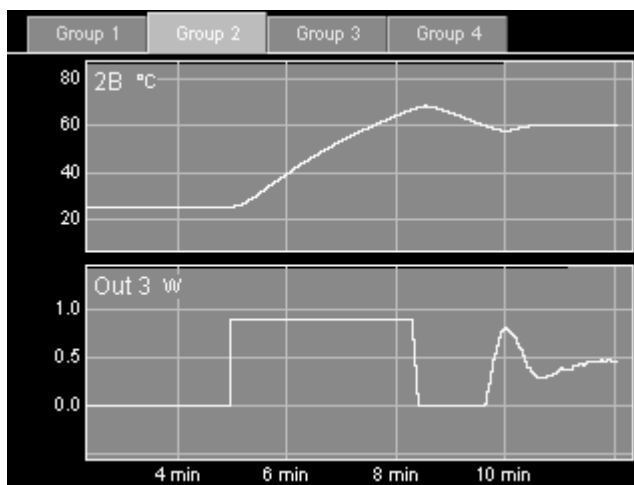
Temperature (top) and heater power (bottom) during step response autotuning. Step Y is 0.9 W, Lag is 10 s, feedback is initially off, and the system starts at room temperature. After the step response is complete, the feedback turns on and stabilizes the system at the 60°C setpoint.
